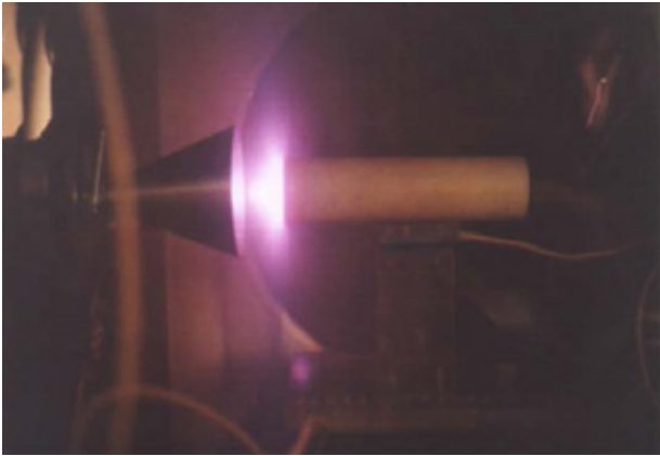
Fig. 1. Laboratory plasma: glow discharge in supersonic air flow.
